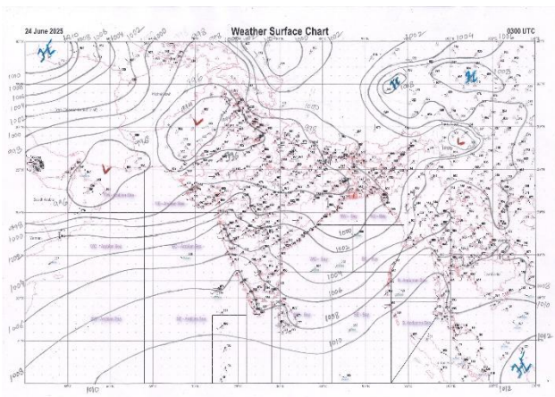
g.1. Analysed surface chart based on 03z observation
